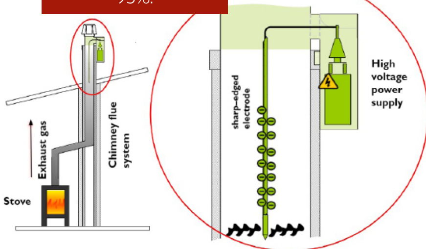
3. The electrostatically charged particles move to the chimney's inner wall.
