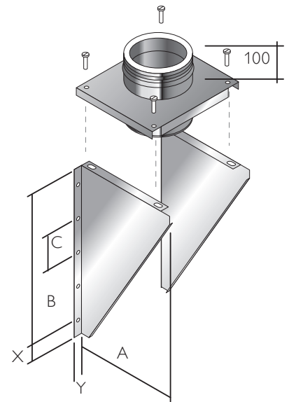
Fig. 2 Top Plate and Side Plates
