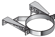
Structural Wall Band with Type W1 Extension Assembly
