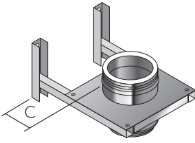
Cantilever Support
